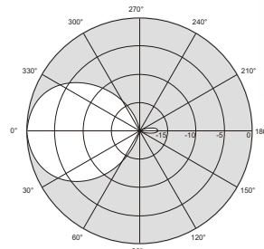
Horizontal Pattern (High Band)
